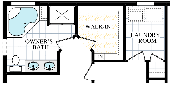
OPTIONAL OWNER'S BATH
