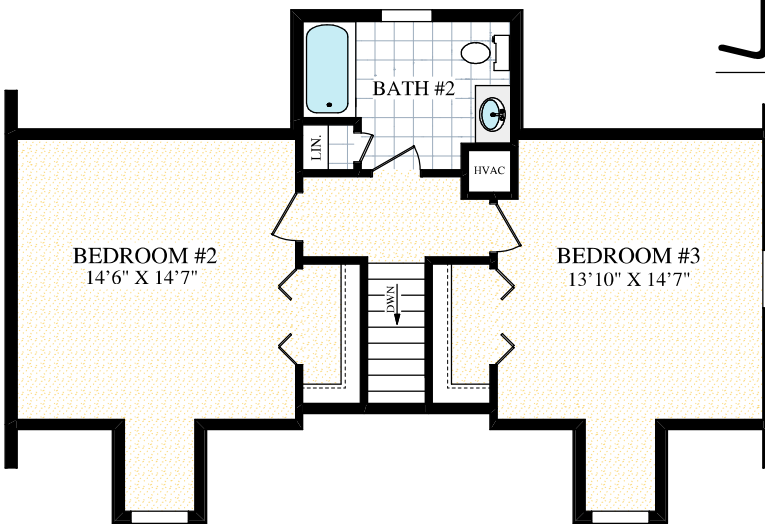
2ND FLOOR LEVEL
