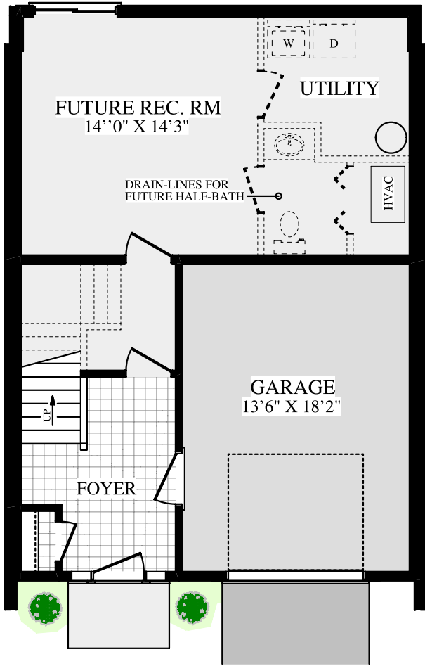
ENTRY LEVEL
